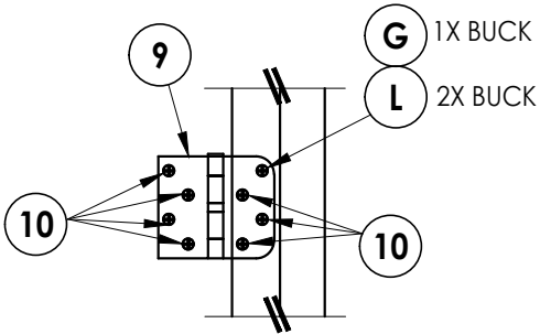
HINGE DETAIL
